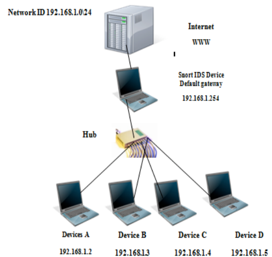
Fig. 5 Snort IDS Network Topology
