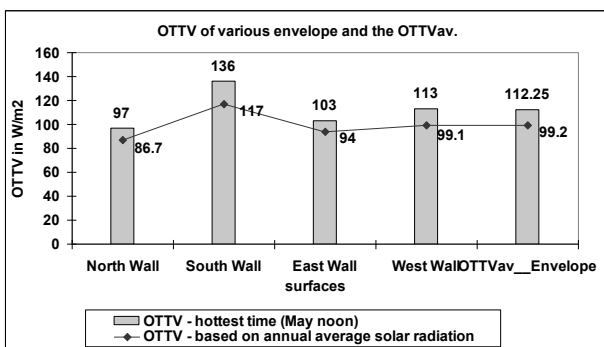
Fig. 2: OTTV of various walls
