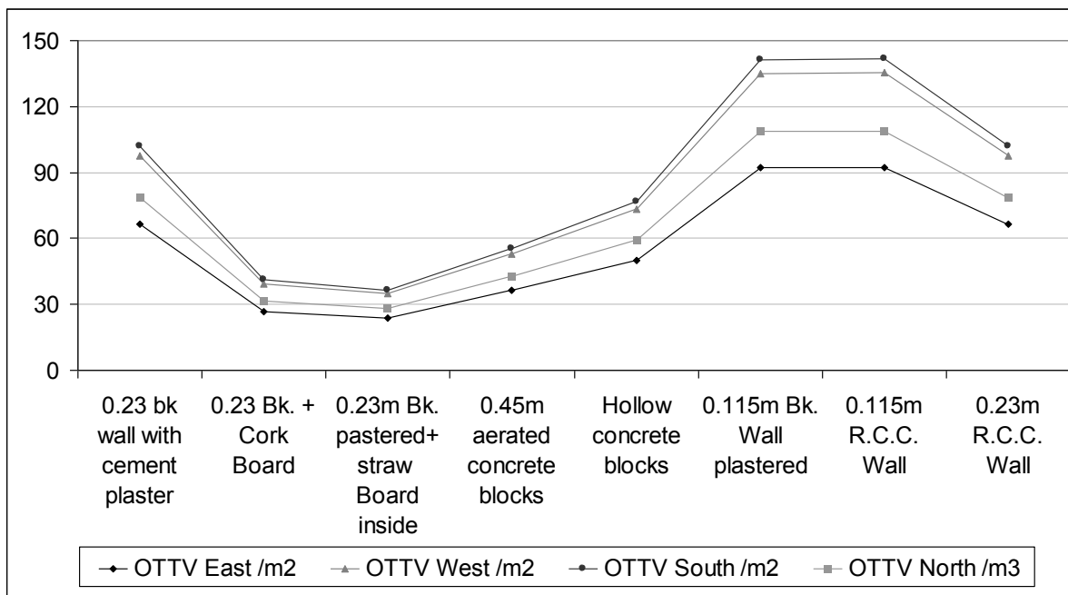
Fig. 4: OTTV for varying walling materials
