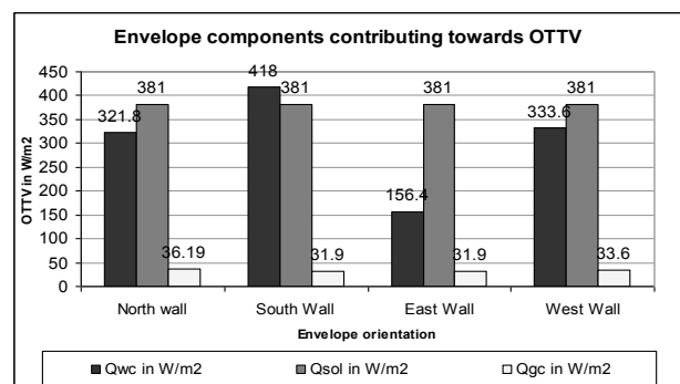
Fig. 3: Envelope component contributing to OTTV
