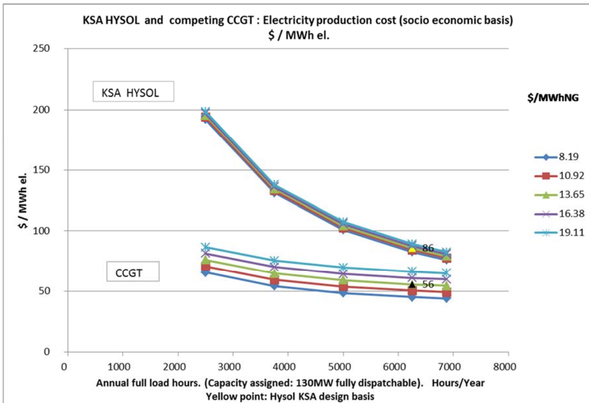
Fig. 4 Electricity production costs for Combined Cycle Gas Turbine (CCGT) and KSA HYSOL configuration, as function of load factor and NG price. Assumed: CO 2 costs = 40 $/tonCO 2 , R=4 %p.a., Lifetime=25 years. Unit: $/MWh el.
