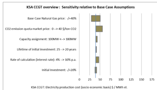
Fig. 7 KSA CCGT results in overview: Electricity production costs (LCOE) - Sensitivity relative to Base Case Assumptions. Units: $/MWh el.
