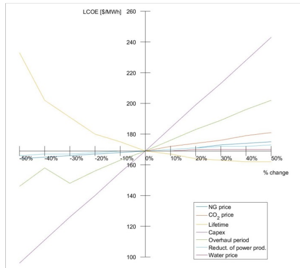
Fig. 9 Sensitivity analysis Private economic: technical parameters
