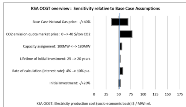
Fig. 6 KSA OCGT results in overview: Electricity production costs (LCOE) - Sensitivity relative to Base Case Assumptions. Units: $/MWh el.
