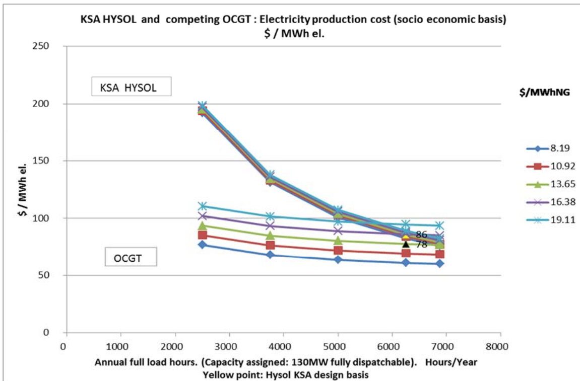
Fig. 2 Electricity production costs for Open Cycle Gas Turbine (OCGT) and KSA HYSOL configuration, as function of load factor and NG price. Assumed: CO 2 costs = 40 $/tonCO 2 , R=4 %p.a., Lifetime=25 years. Unit: $/MWh el.
