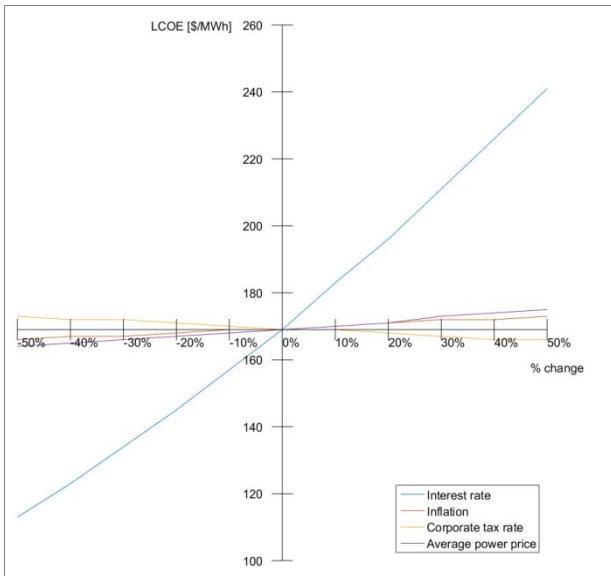
Fig. 8 Sensitivity analysis Private economic: economic parameters
