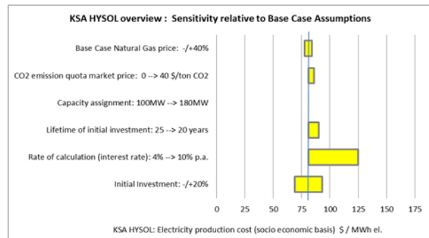
Fig. 5 KSA HYSOL results in overview: Electricity production costs (LCOE) - Sensitivity relative to Base Case Assumptions. Units: $/MWh el
