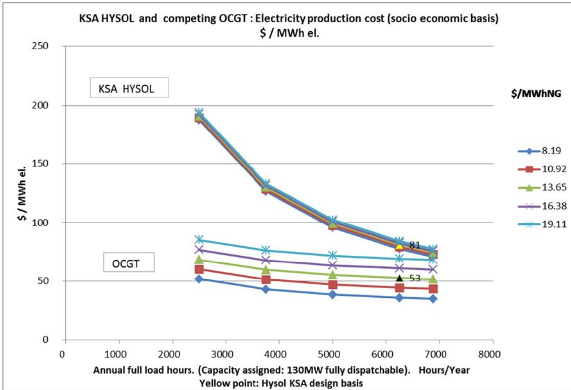
Fig. 1 Electricity production costs for Open Cycle Gas Turbine (OCGT) and KSA HYSOL configuration, as function of load factor and NG price. Assumed: CO 2 costs = 0 $/ton CO 2 , R=4 %p.a., Lifetime=25 years. Unit: $/MWh el
