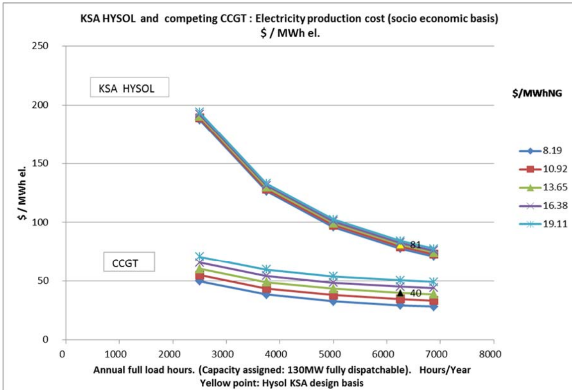
Fig. 3 Electricity production costs for Combined Cycle Gas Turbine (CCGT) and KSA HYSOL configuration, as function of load factor and NG price. Assumed: CO 2 costs = 0 $/tonCO 2 , R= 4%p.a., Lifetime=25 years. Unit: $/MWh el.
