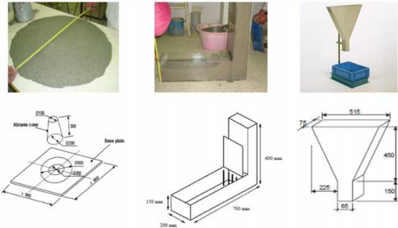
Fig. 4. Slump flow, L-box and V-funnel
