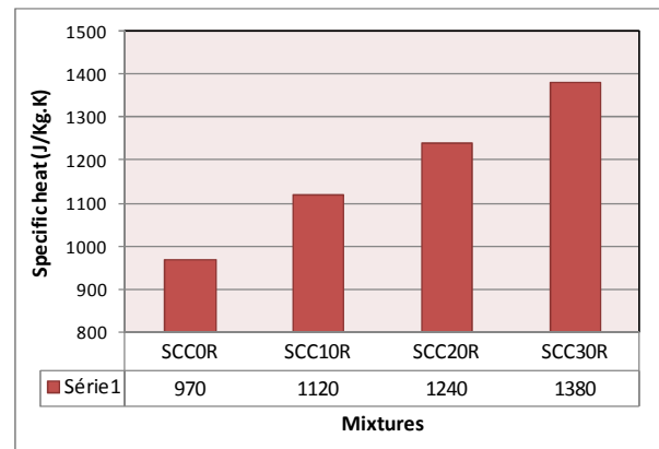
Fig. 13. Effect of rubber aggregates on the specific heat
