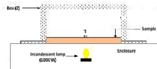
Fig. 6. Thermal diffusivity testing apparatus
