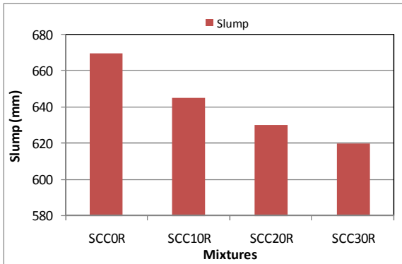
Fig. 7. Slump flow test
