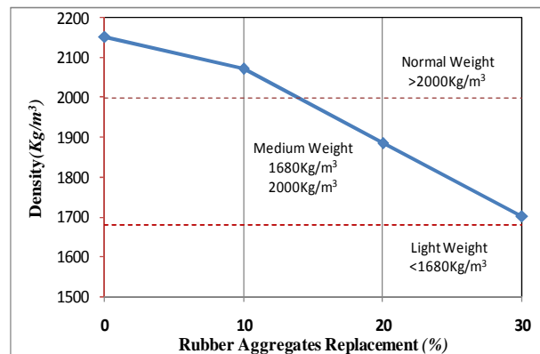
Fig. 10. Effect of rubber aggregates on the dry density
