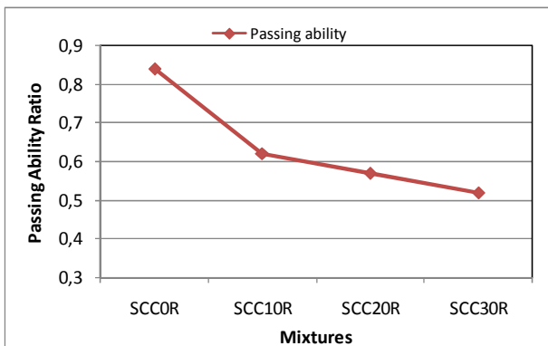
Fig. 8. L-box test (Passing Ability)
