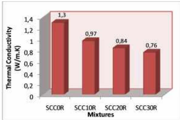
Fig. 11. Effect of rubber aggregates on the thermal conductivity
