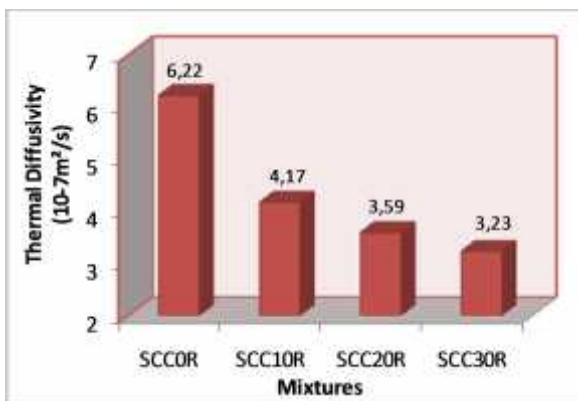
Fig. 12. Effect of rubber aggregates on the thermal diffusivity
