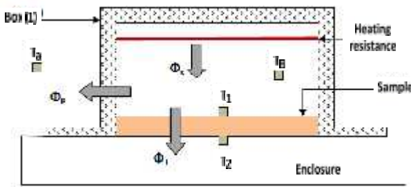
Fig. 5. Thermal conductivity testing apparatus
