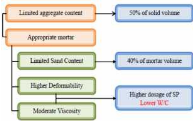
Fig. 3. Methods of achieving self compactability
