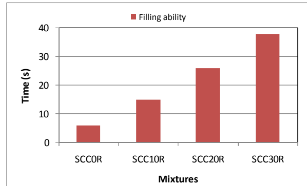
Fig. 9. Filling ability for the mixtures
